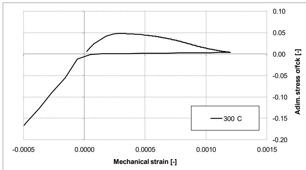
Figure 13 : Transition zone between tension and compression
