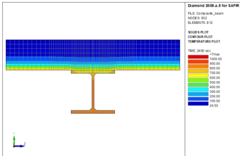
Figure 11: composite steel-concrete beam, isotherm after 2400 seconds
