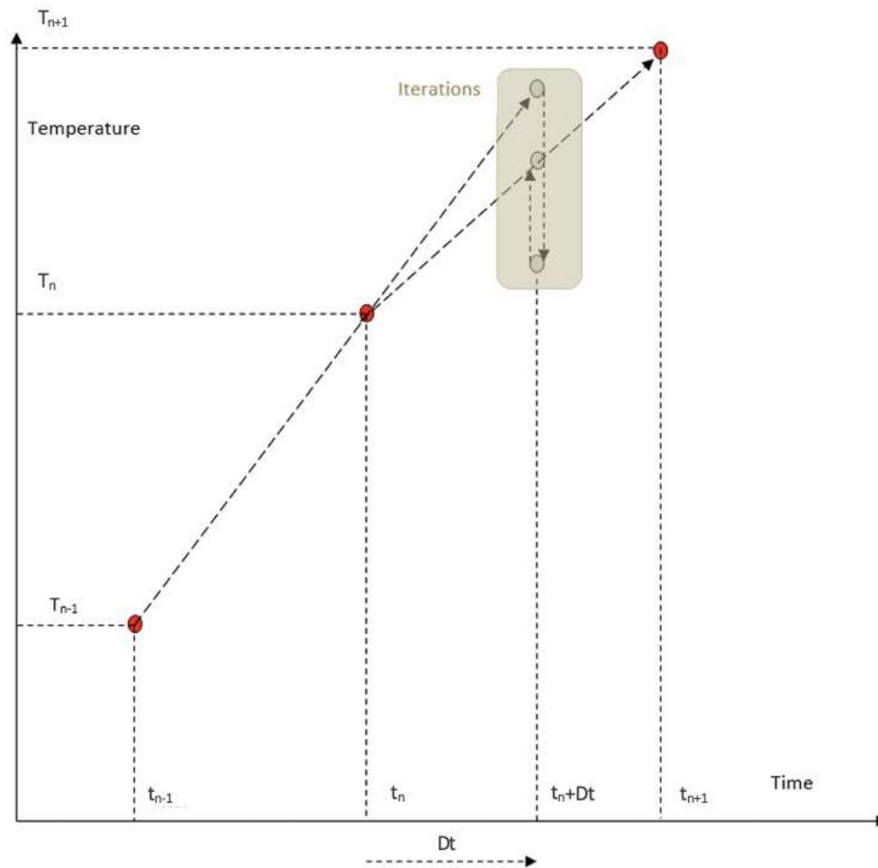
Figure 3: graphic representation of the iterations performed within one time step
