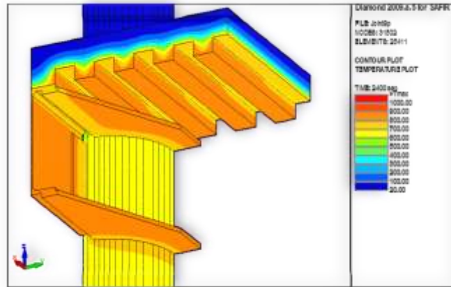
Figure 10: composite steel-concrete joint 7
