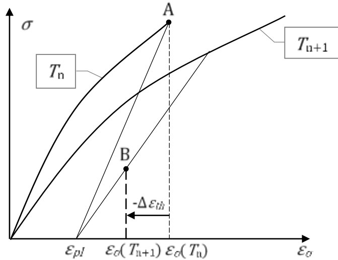
Figure 4: evolution during the first iteration
