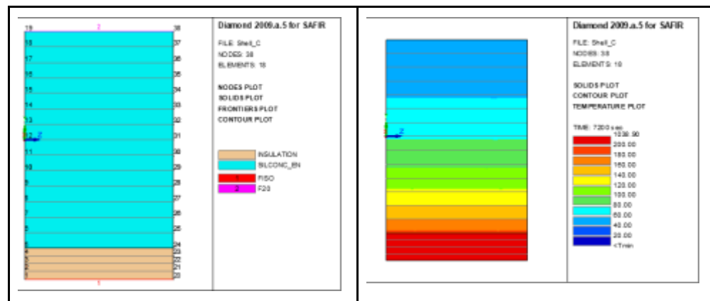
Figure 12: concrete shell protected on the bottom face
