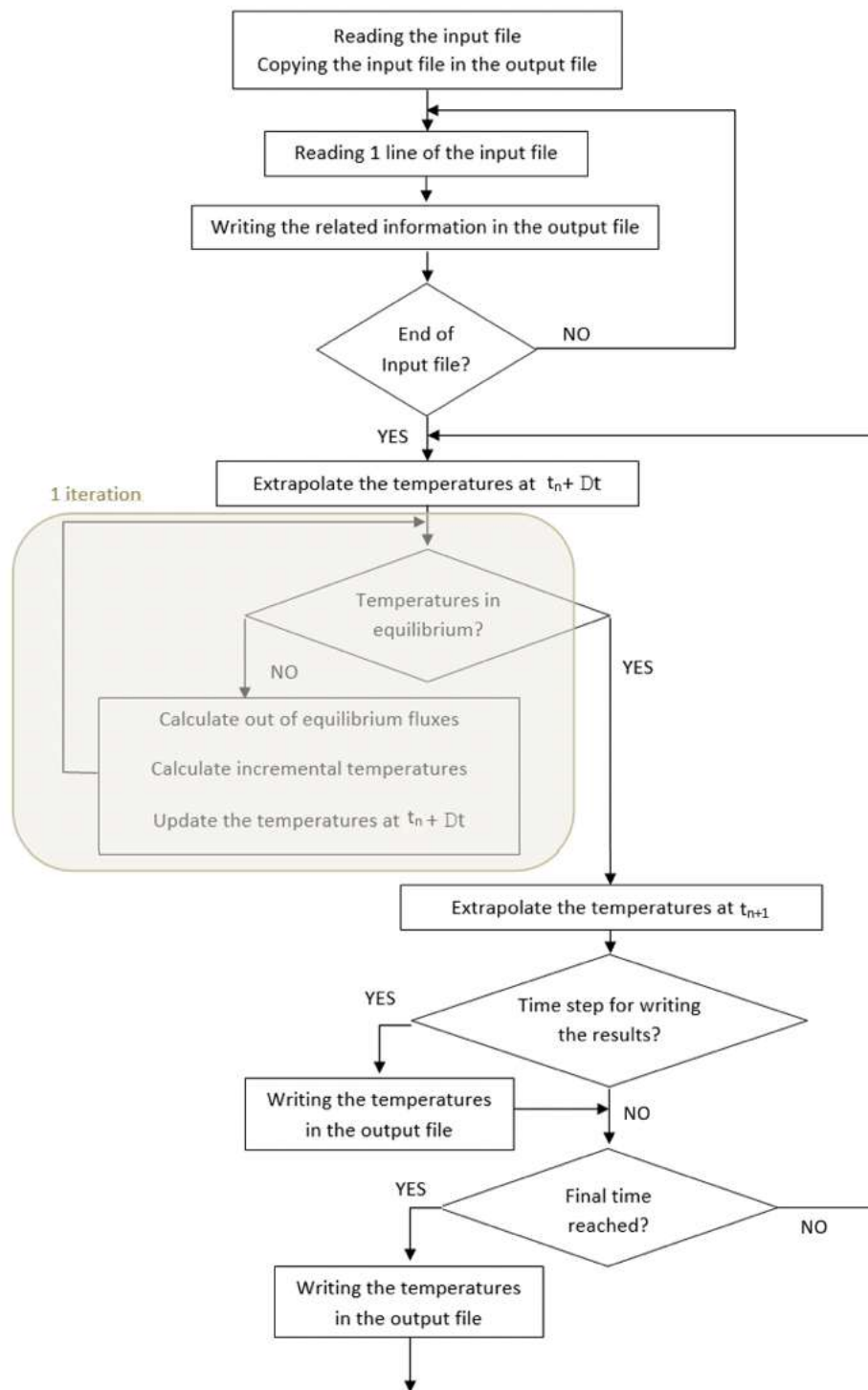
Figure 2: graphic representation of the algorithm for a thermal calculation
